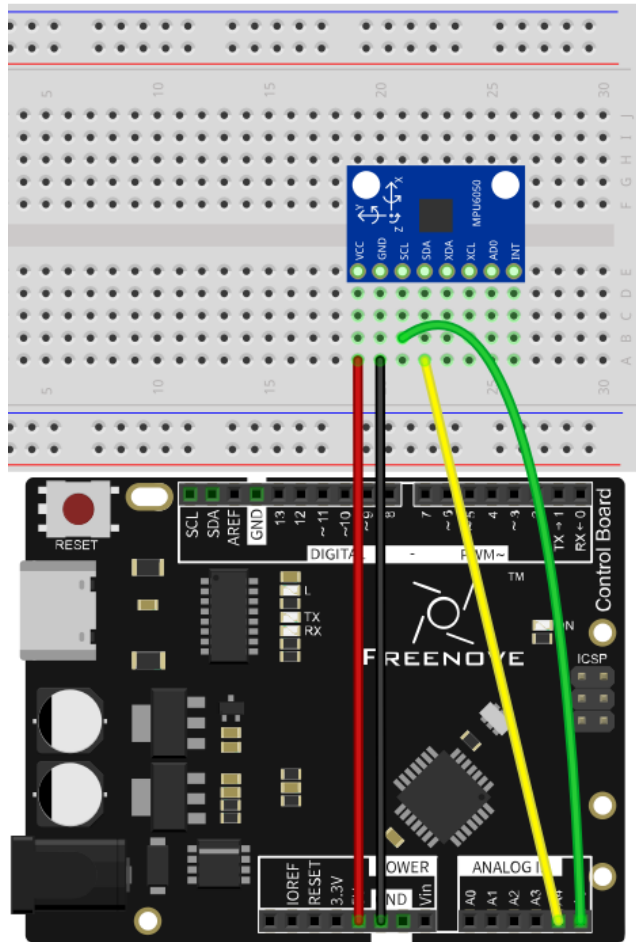
Hardware connection
