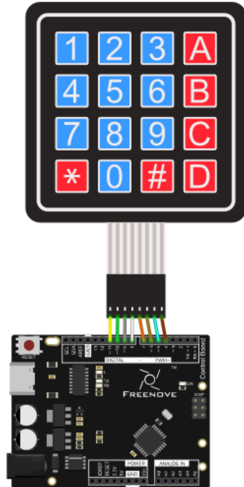
Hardware connection
