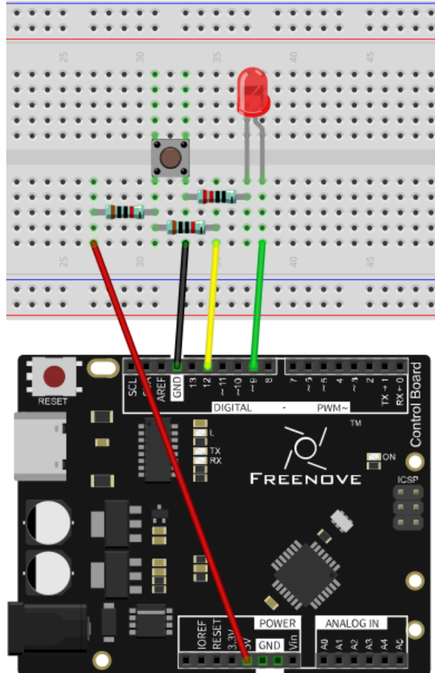
Hardware Connection
